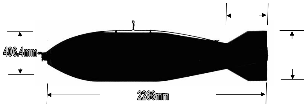
750lb M117 HE GP fitted with a fragmentation kit.
